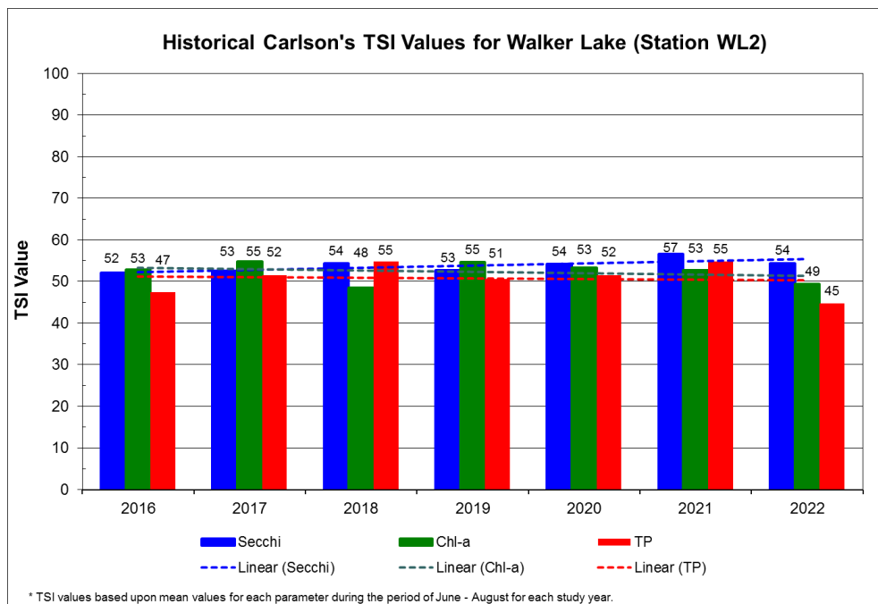
Figure 4.12 Carlson’s TSI Values for Station WL2 (2016-2022)
