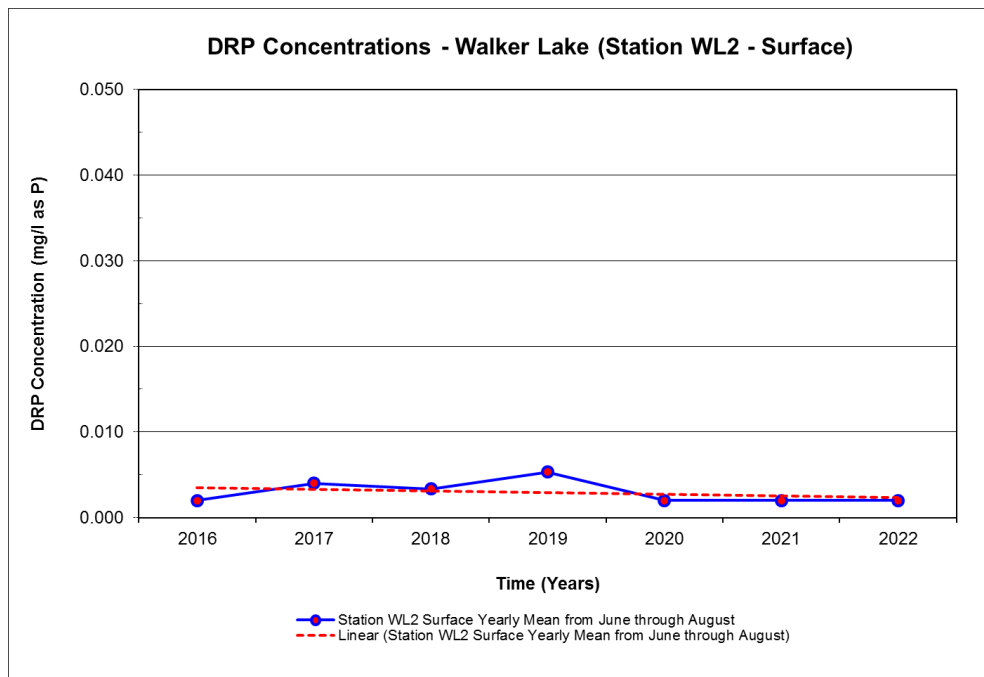
Figure 4.4 Dissolved Reactive Phosphorus Concentrations in Walker Lake (2016-2022)
