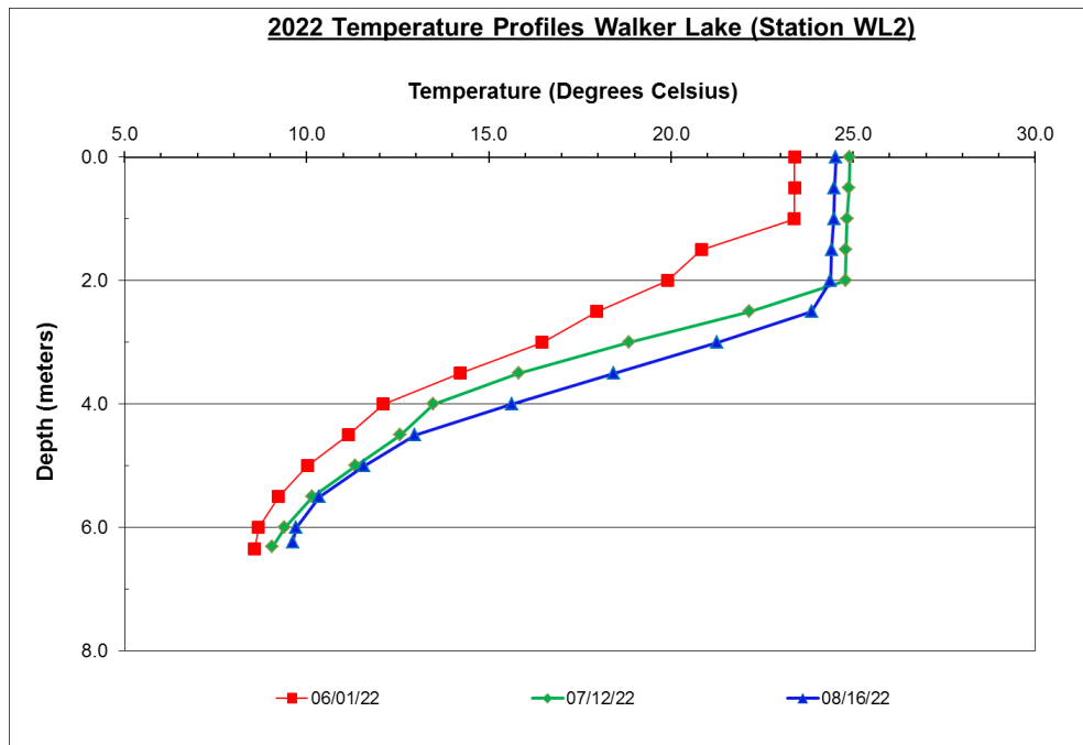
Figure 4.1 2022 Temperature Profiles in Walker Lake at Station WL2
