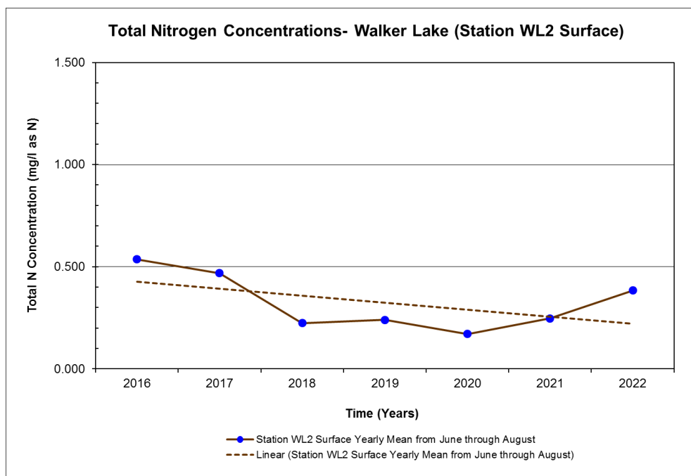
Figure 4.5 Total Nitrogen Concentrations in Walker Lake (2016-2022)
