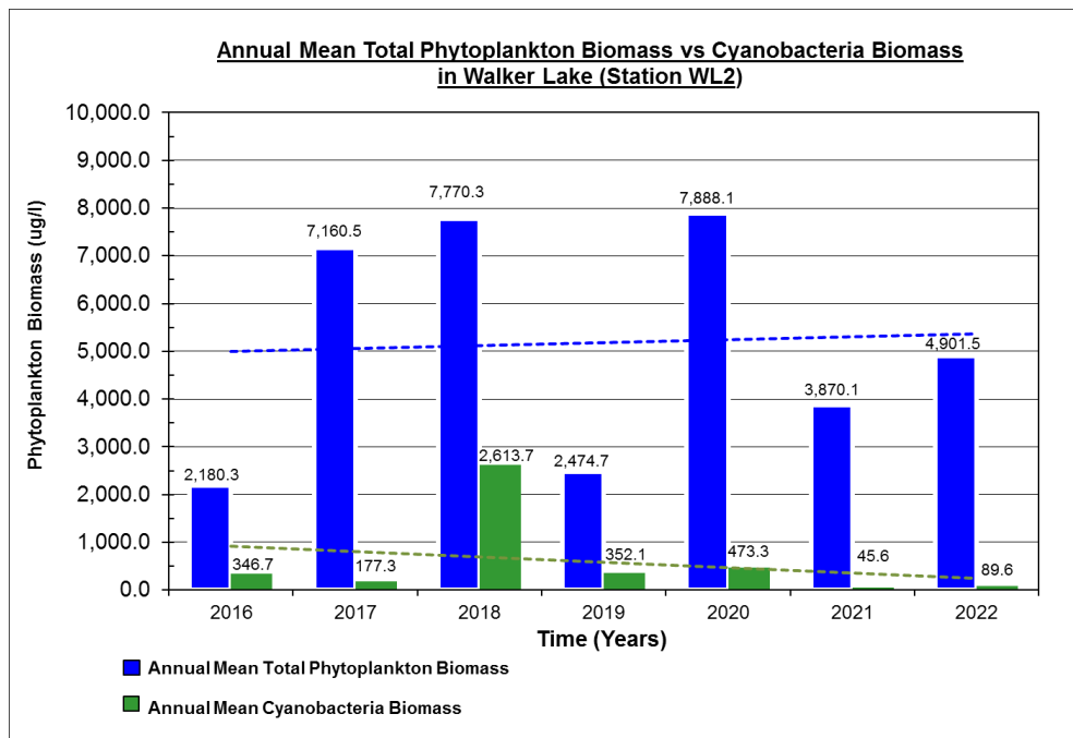
Figure 4.9 Mean Phytoplankton vs. Cyanobacteria Biomass in Walker Lake (2016-2022)
