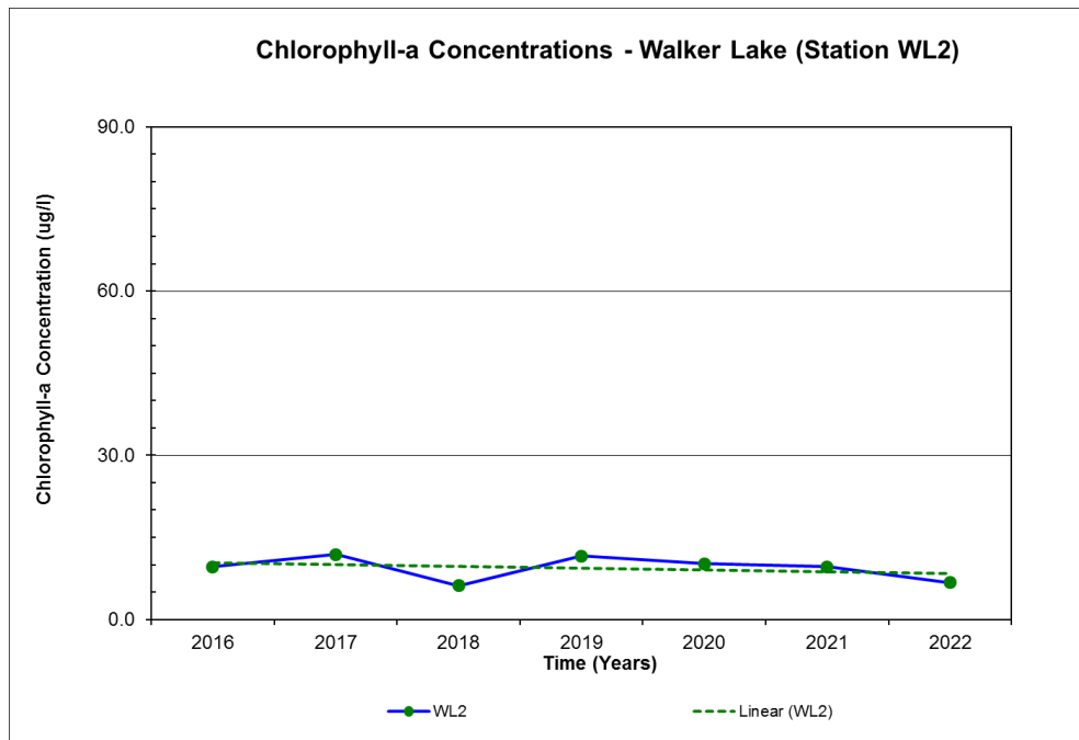
Figure 4.7 Chlorophyll-a Concentrations in Walker Lake (2016-2022)
