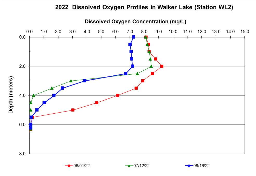
Figure 4.2 2022 Dissolved Oxygen Profiles in Walker Lake at Station WL2
