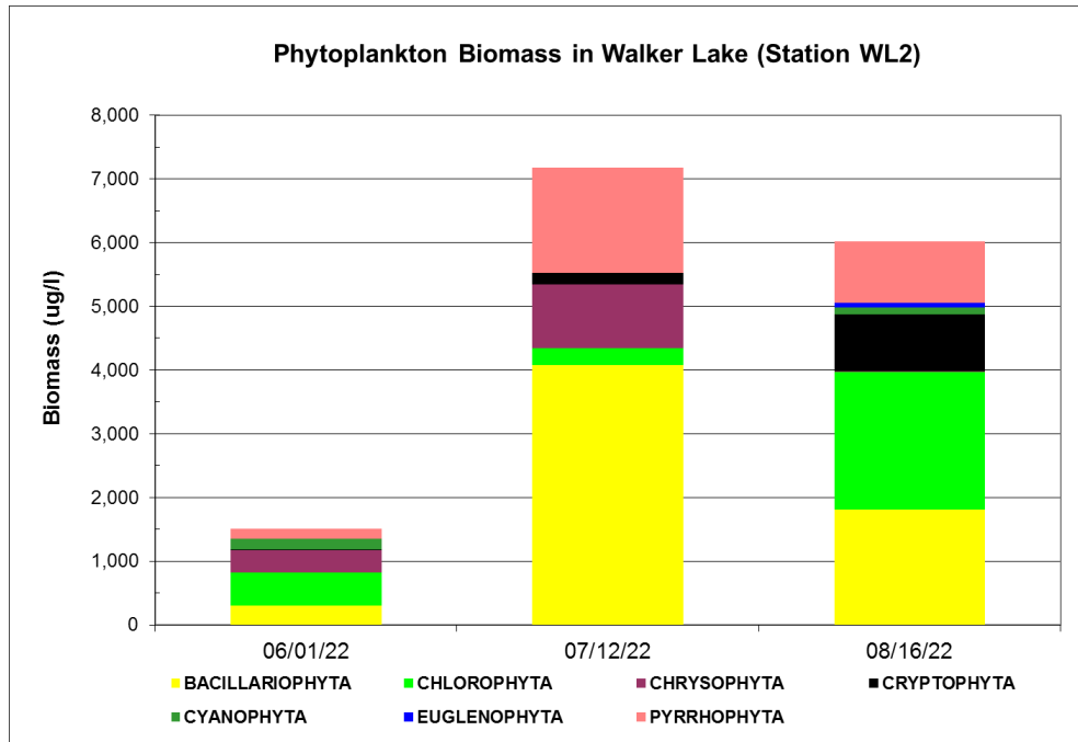
Figure 4.8 Phytoplankton Biomass in Walker Lake in 2022
