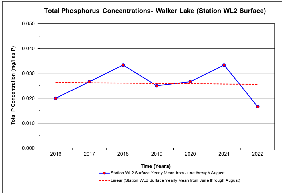
Figure 4.3 Total Phosphorus Concentrations in Walker Lake (2016-2022)
