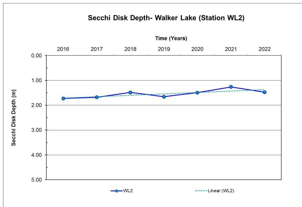
Figure 4.6 Secchi Disk Transparency in Walker Lake (2016-2022)
