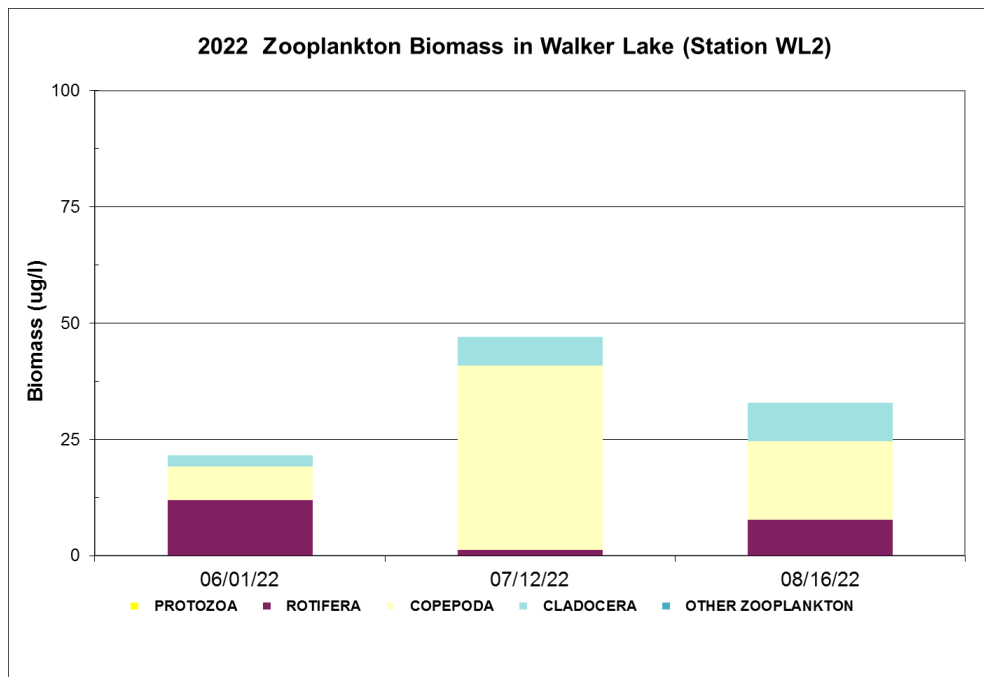
Figure 4.10 Zooplankton Biomass in Walker Lake in 2022
