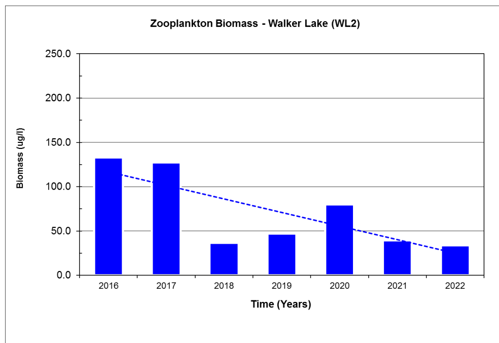
Figure 4.11 Mean Zooplankton Biomass in Walker Lake (2016-2022)
