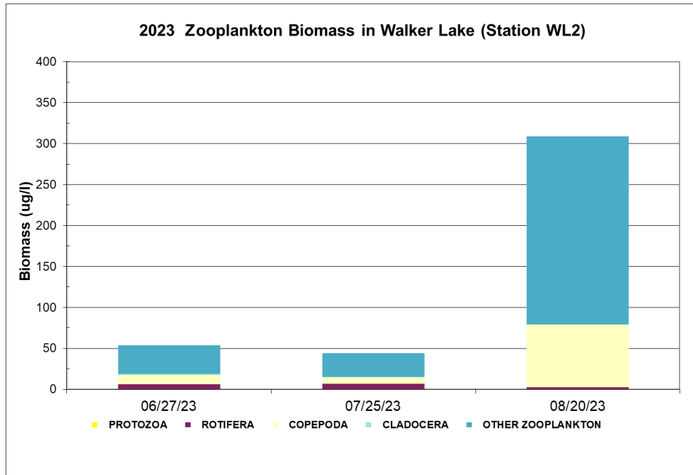
Figure 4.10 Zooplankton Biomass in Walker Lake in 2023
