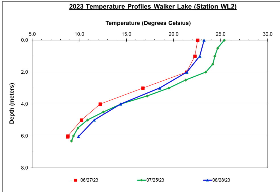
Figure 4.1 2023 Temperature Profiles in Walker Lake at Station WL2
