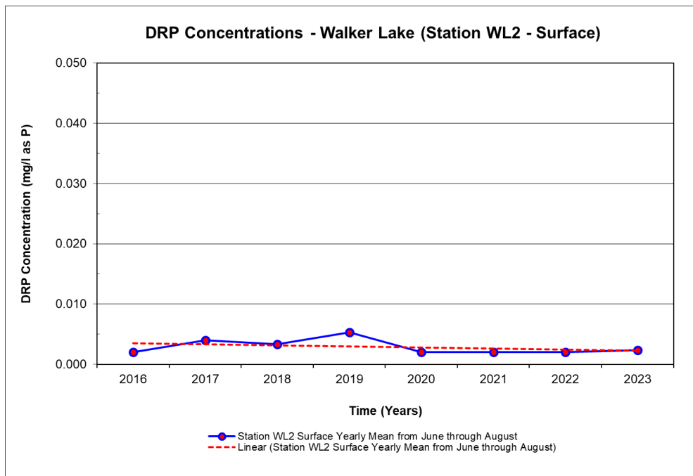
Figure 4.4 Dissolved Reactive Phosphorus Concentrations in Walker Lake (2016-2023)
