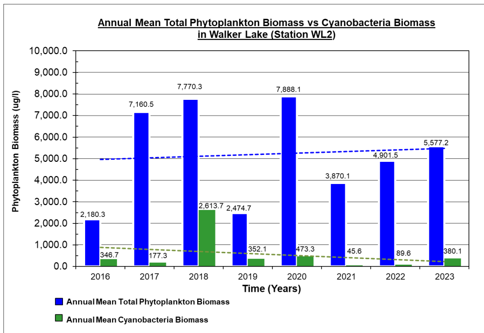
Figure 4.9 Mean Phytoplankton vs. Cyanobacteria Biomass in Walker Lake (2016-2023)
