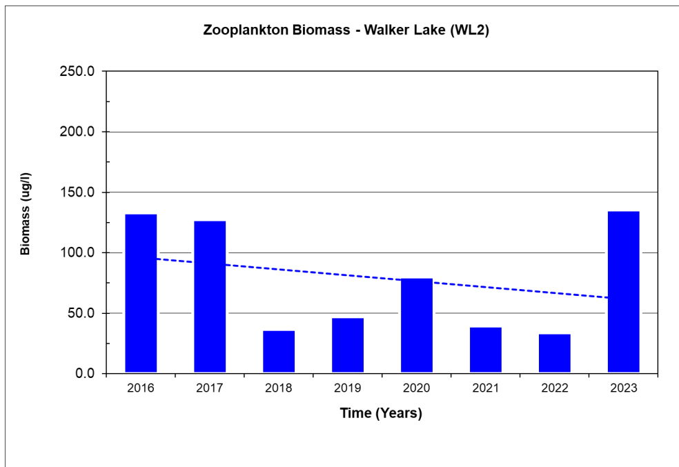
Figure 4.11 Mean Zooplankton Biomass in Walker Lake (2016-2023)
