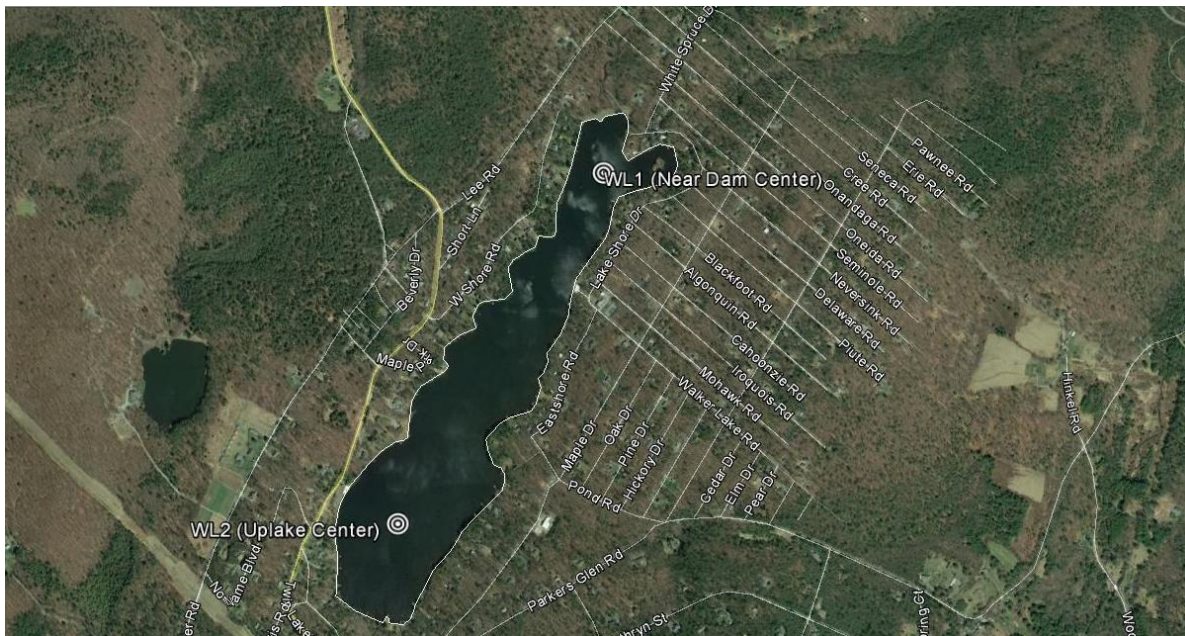
Figure 1.1 Walker Lake & Locations of Lake Monitoring Stations
