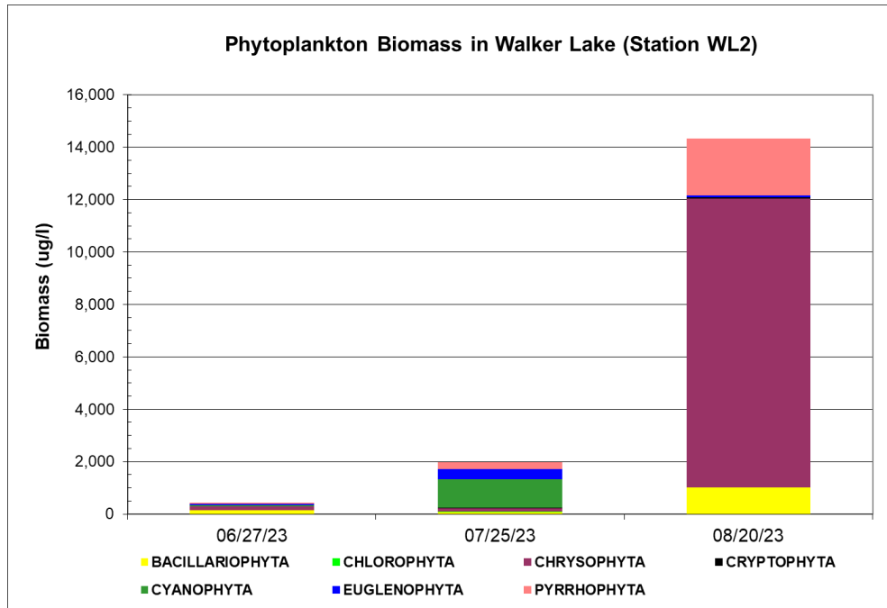
Figure 4.8 Phytoplankton Biomass in Walker Lake in 2023
