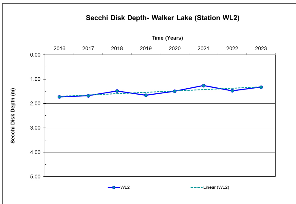
Figure 4.6 Secchi Disk Transparency in Walker Lake (2016-2023)
