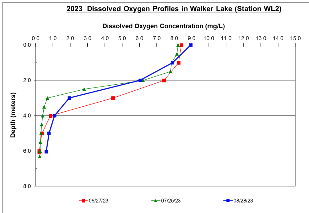
Figure 4.2 2023 Dissolved Oxygen Profiles in Walker Lake at Station WL2
