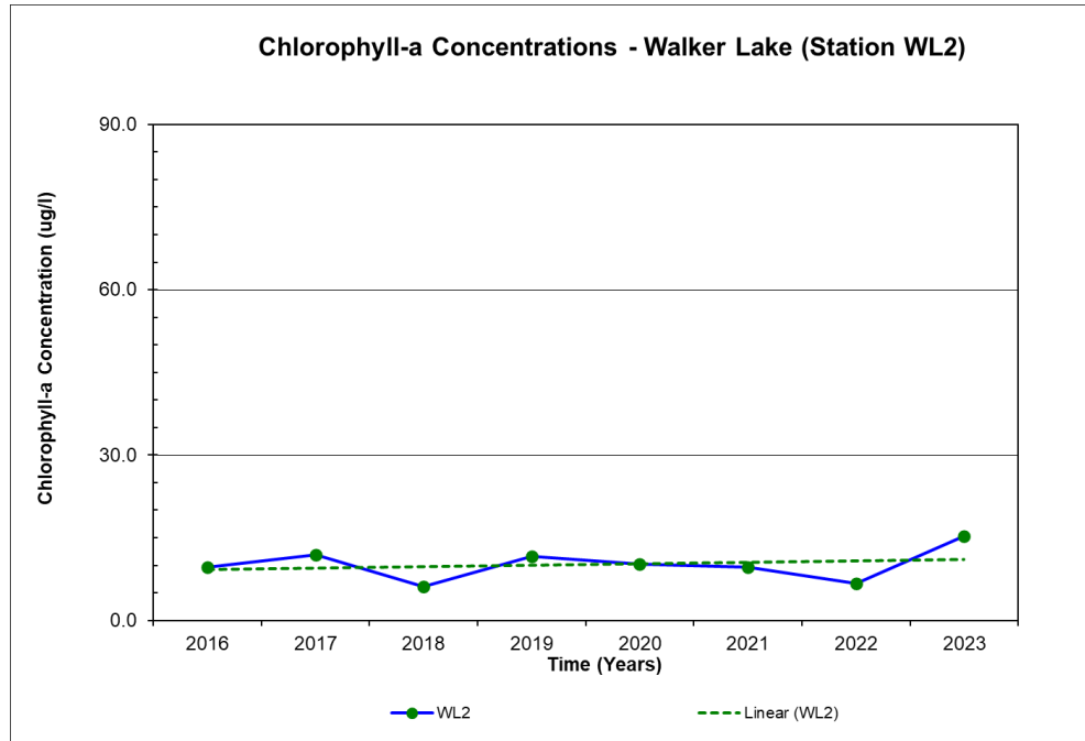
Figure 4.7 Chlorophyll-a Concentrations in Walker Lake (2016-2023)
