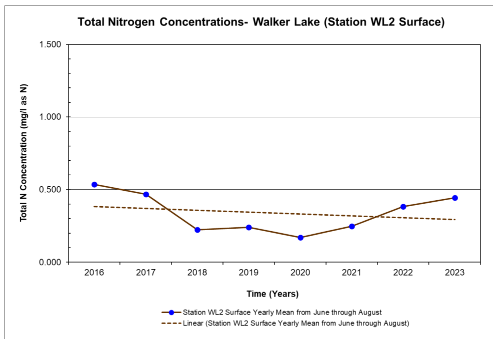
Figure 4.5 Total Nitrogen Concentrations in Walker Lake (2016-2023)
