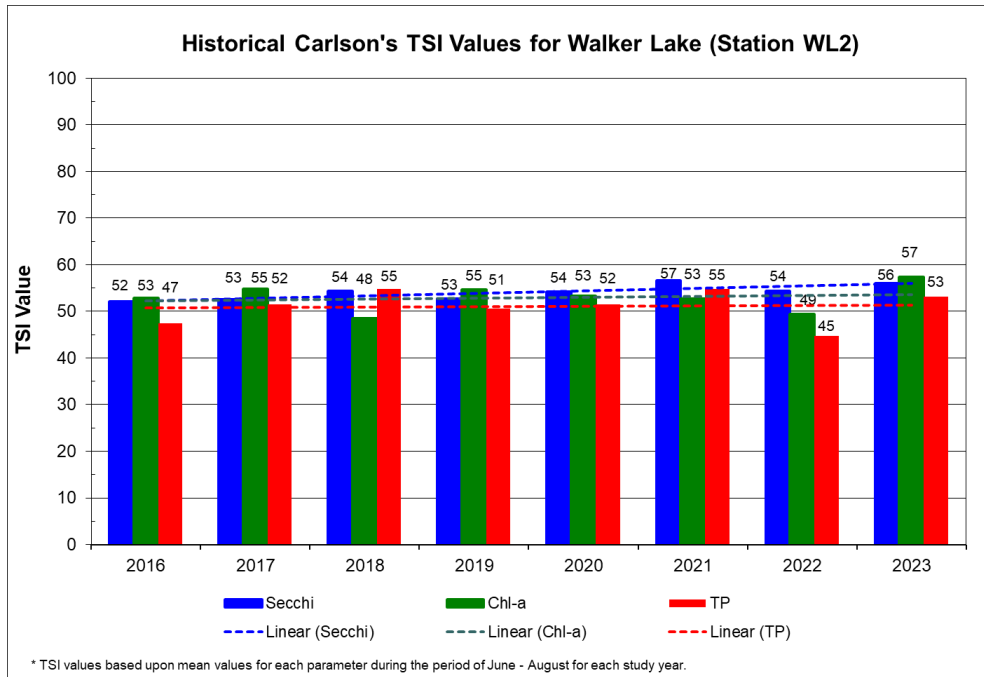
Figure 4.12 Carlson's TSI Values for Station WL2 (2016-2023)
