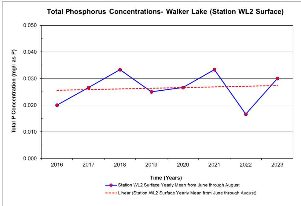
Figure 4.3 Total Phosphorus Concentrations in Walker Lake (2016-2023)
